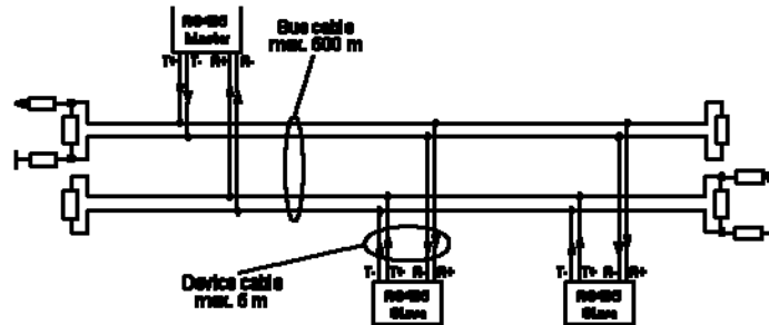
FIGURE 5: RS485 4-WIRE INTERFACE SETUP 6
